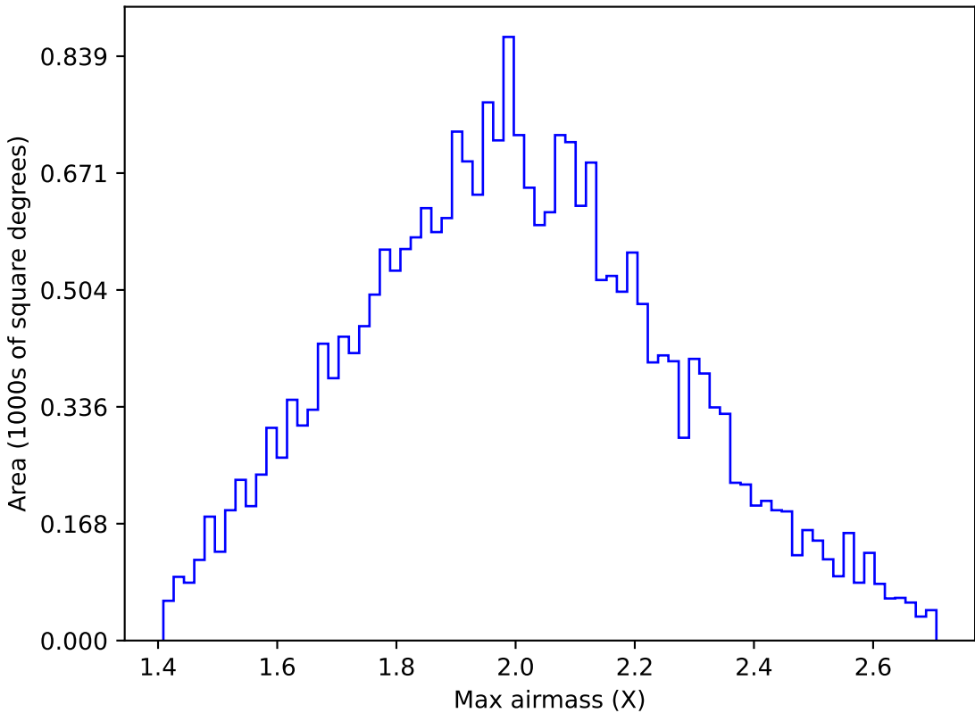
ddf_acor_sf10_lsf15_lsr10_v3.4_10yrs All sky g band: Max airmass
