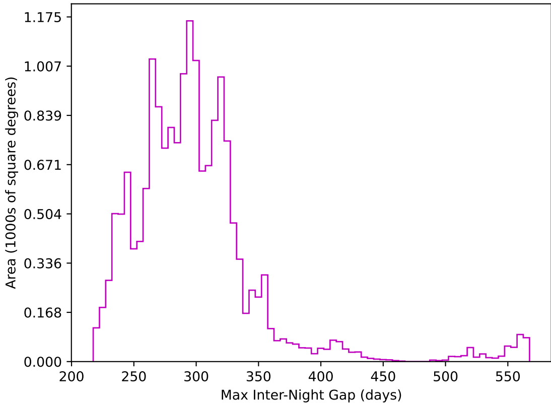
ddf_acor_sf10_lsf15_lsr10_v3.4_10yrs WFD z band: Max Inter-Night Gap
