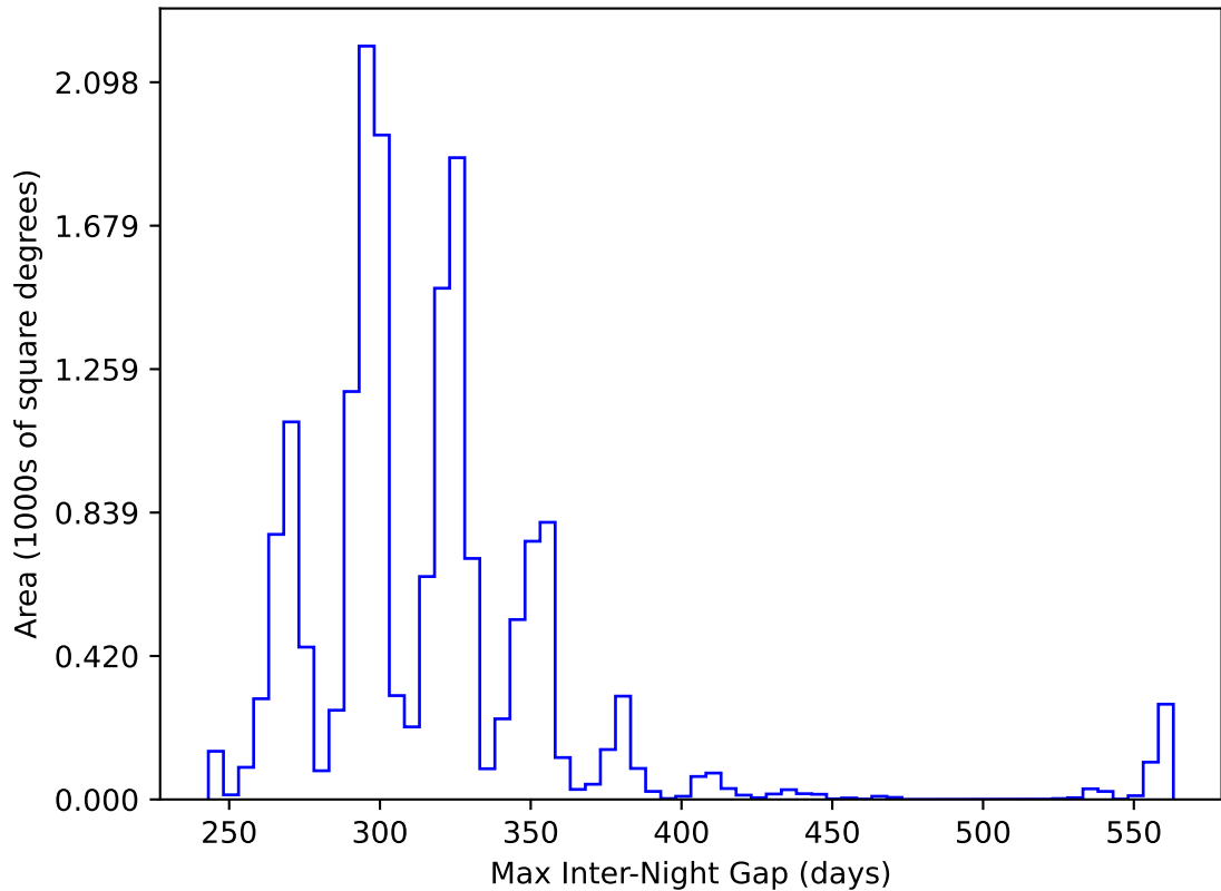
ddf_acor_sf10_lsf15_lsr10_v3.4_10yrs WFD y band: Max Inter-Night Gap
