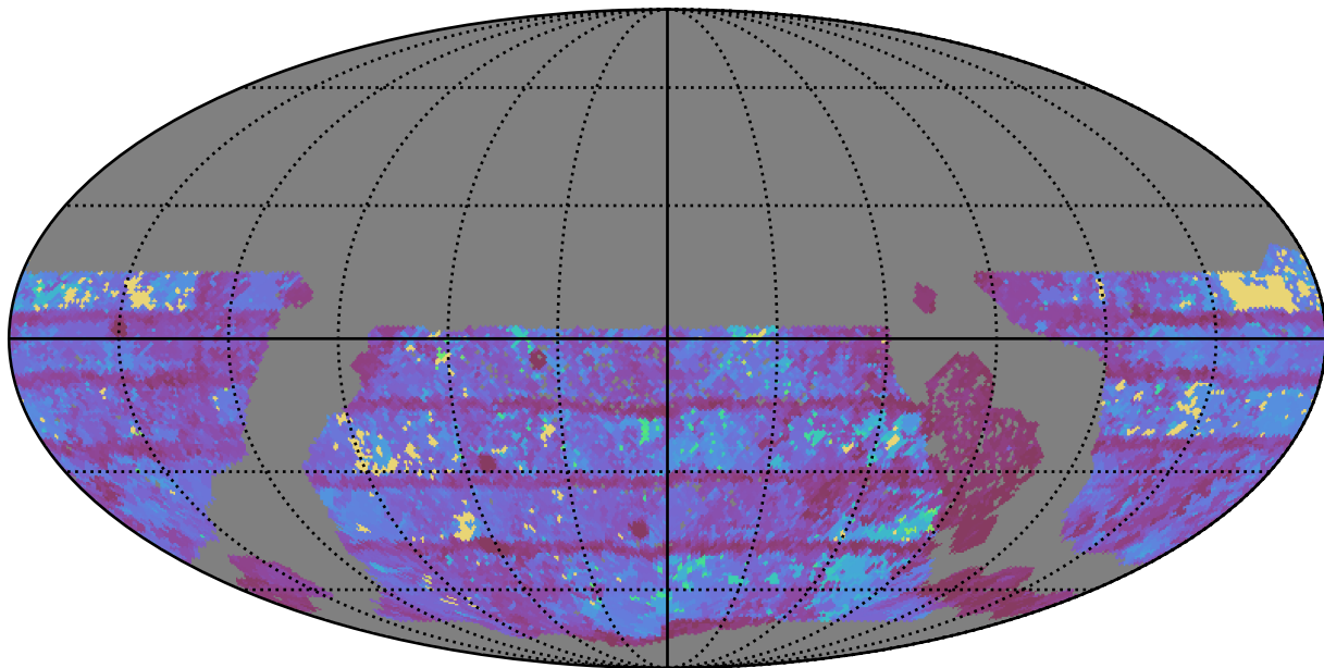
ddf_acor_sf10_ls15_lsr10_v3.4_10yrs WFD r band: Max Inter-Night Gap
