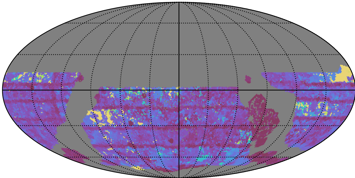
ddf_acor_sf10_lsf15_lsr10_v3.4_10yrs WFD i band: Max Inter-Night Gap
