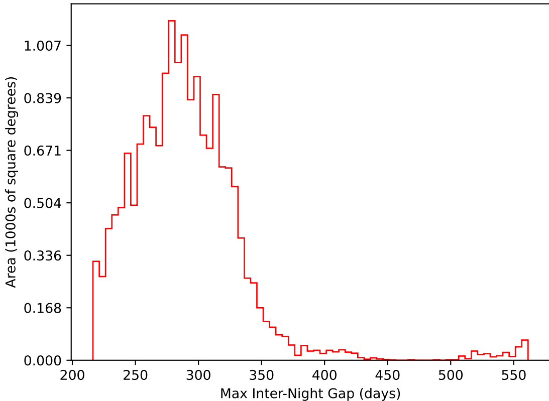
ddf_acor_sf10_ls15_lsr10_v3.4_10yrs WFD i band: Max Inter-Night Gap
