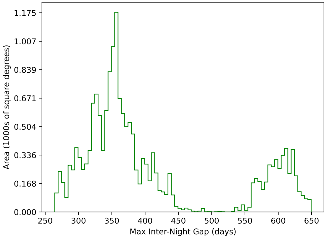
ddf_acor_sf10_lsf15_lsr10_v3.4_10yrs WFD g band: Max Inter-Night Gap
