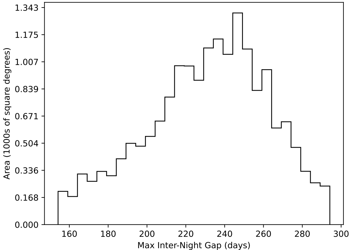
ddf_acor_sf10_lsf15_lsr10_v3.4_10yrs WFD all bands: Max Inter-Night Gap
