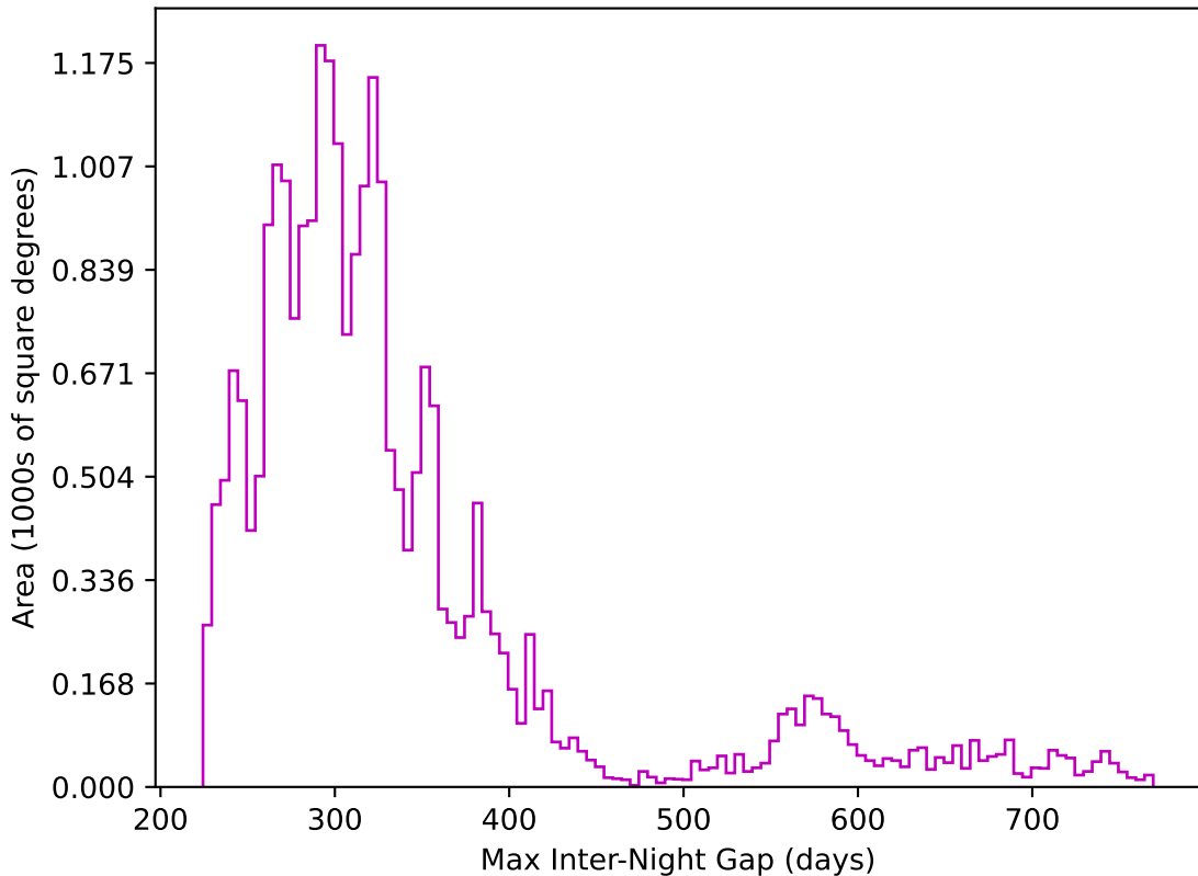
ddf_acor_sf10_lsf15_lsr10_v3.4_10yrs All sky z band: Max Inter-Night Gap
