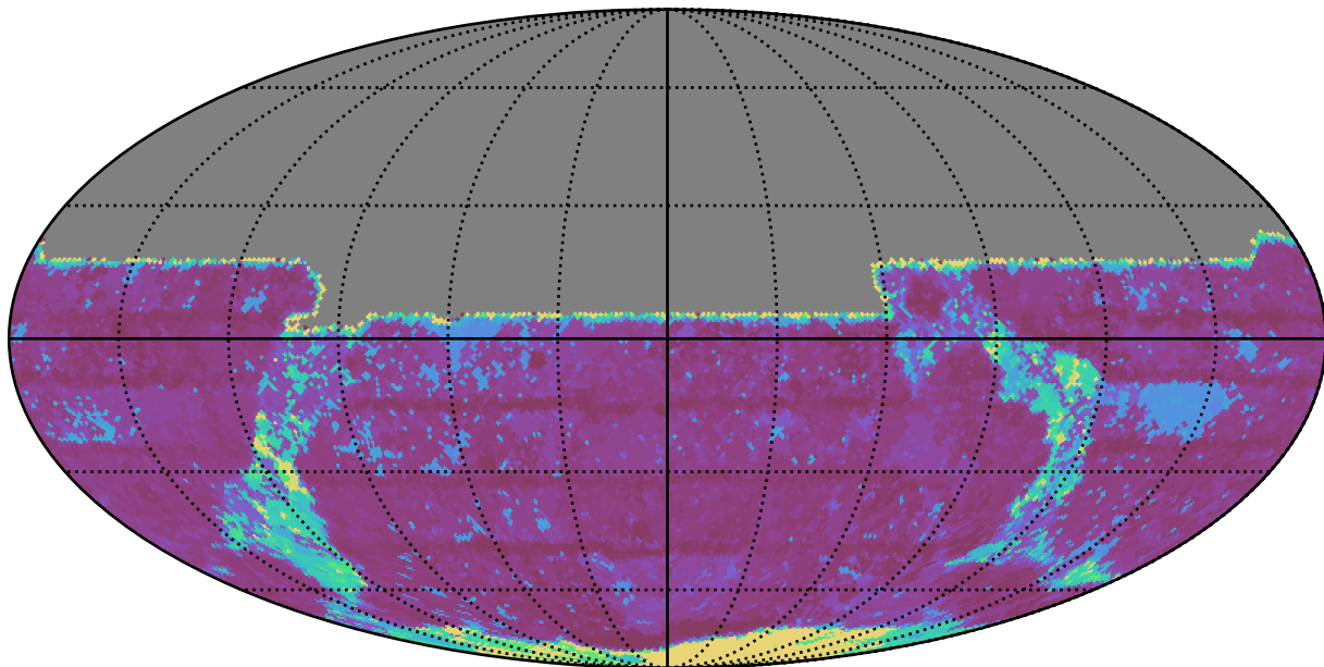
ddf_acor_sf10_lsf15_lsr10_v3.4_10yrs All sky y band: Max Inter-Night Gap
