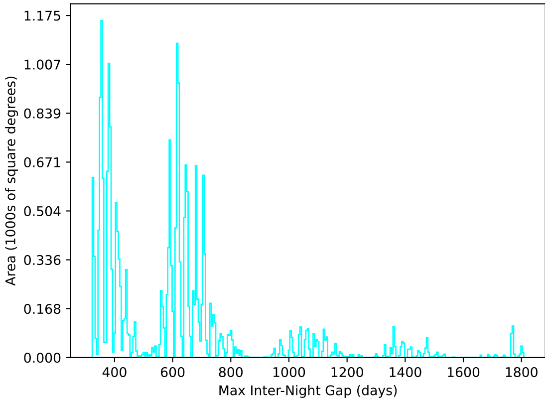
ddf_acor_sf10_lsf15_lsr10_v3.4_10yrs All sky u band: Max Inter-Night Gap
