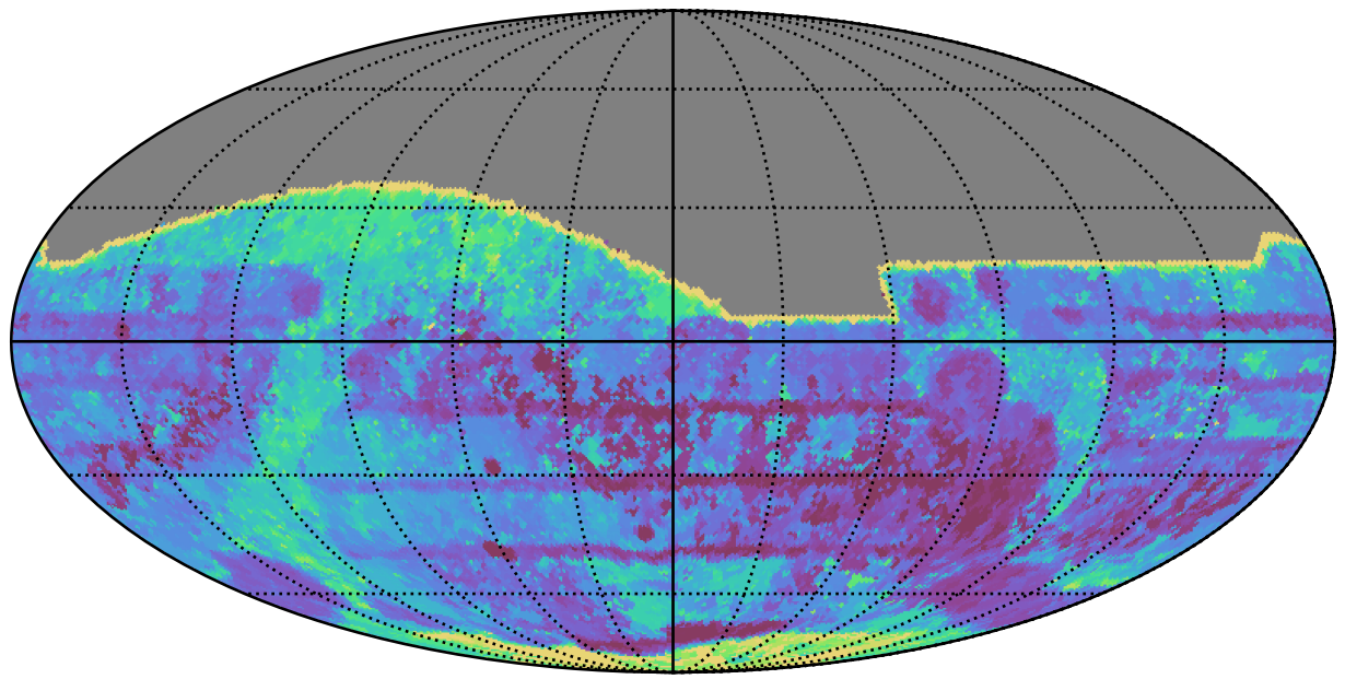
ddf_acor_sf10_lsf15_lsr10_v3.4_10yrs All sky all bands: Max Inter-Night Gap
