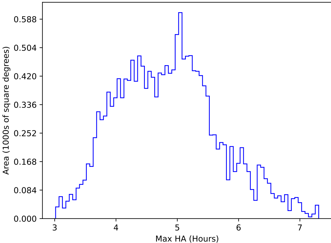
ddf_acor_sf10_lsf15_lsr10_v3.4_10yrs WFD i band: Max HA
