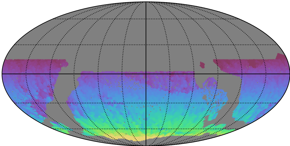
ddf_acor_sf10_lsf15_lsr10_v3.4_10yrs WFD all bands: Max HA
