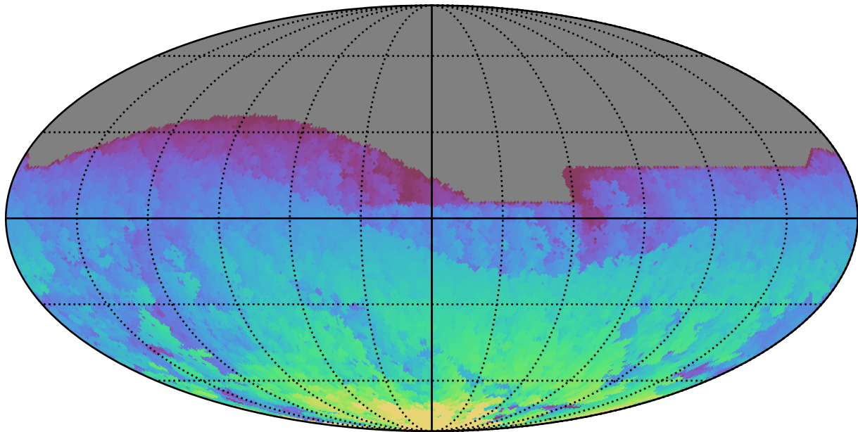
ddf_acor_sf10_lsf15_lsr10_v3.4_10yrs All sky z band: Max HA
