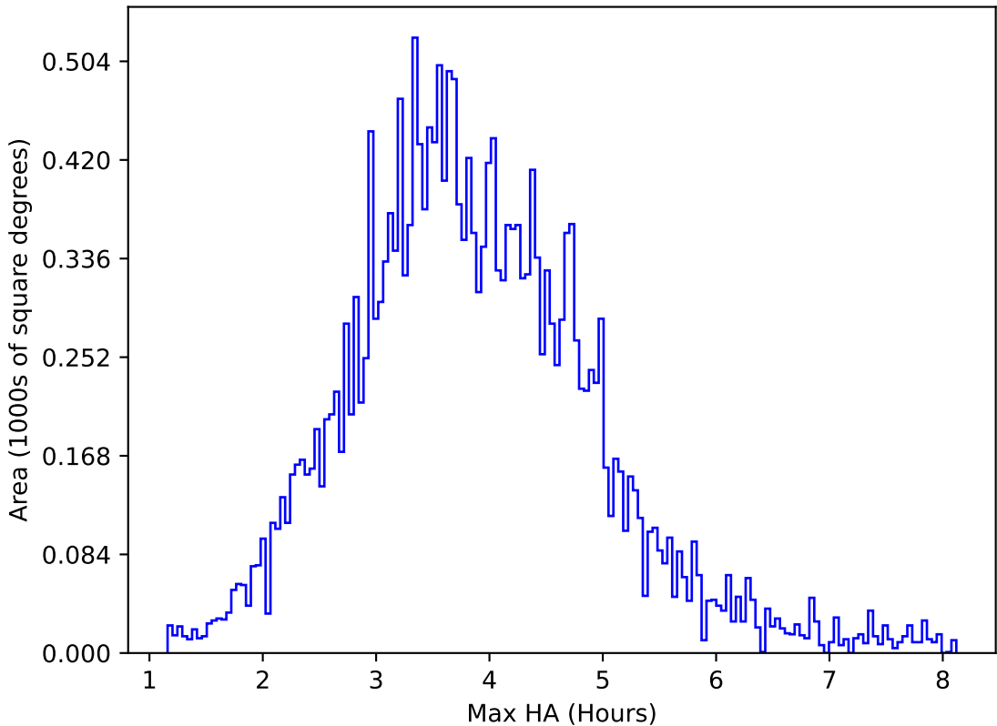
ddf_acor_sf10_lsf15_lsr10_v3.4_10yrs All sky u band: Max HA
