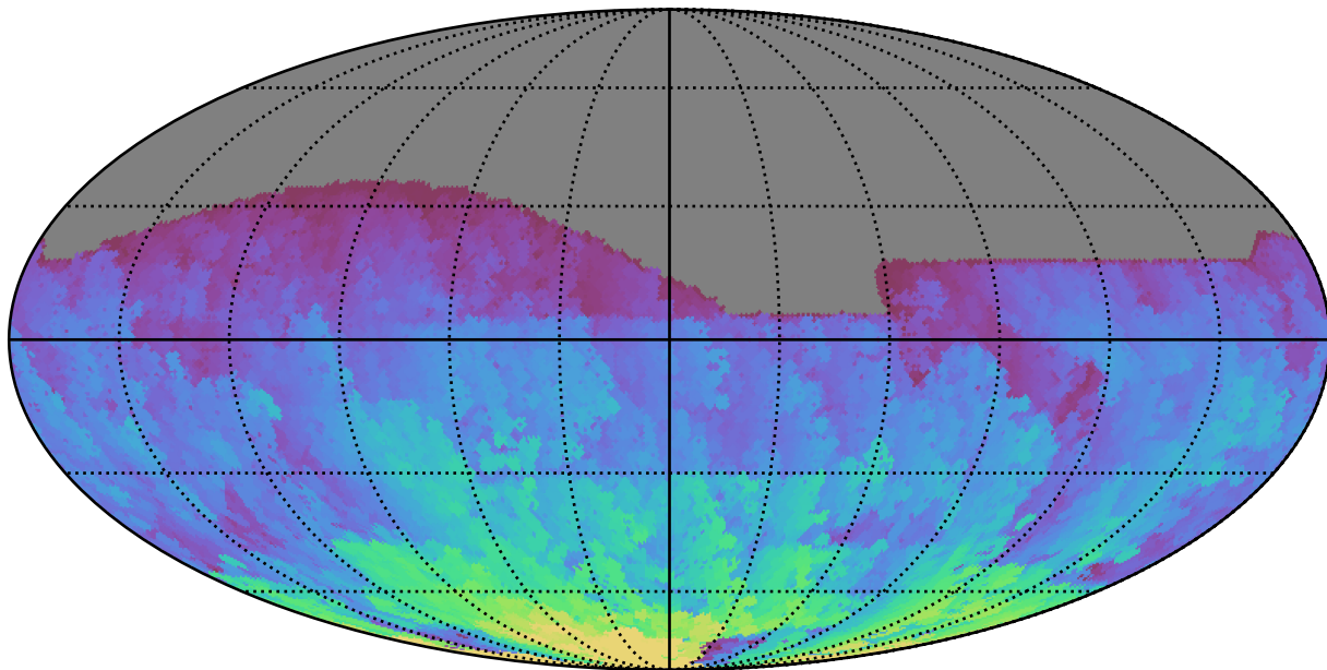
ddf_acor_sf10_lsf15_lsr10_v3.4_10yrs All sky r band: Max HA
