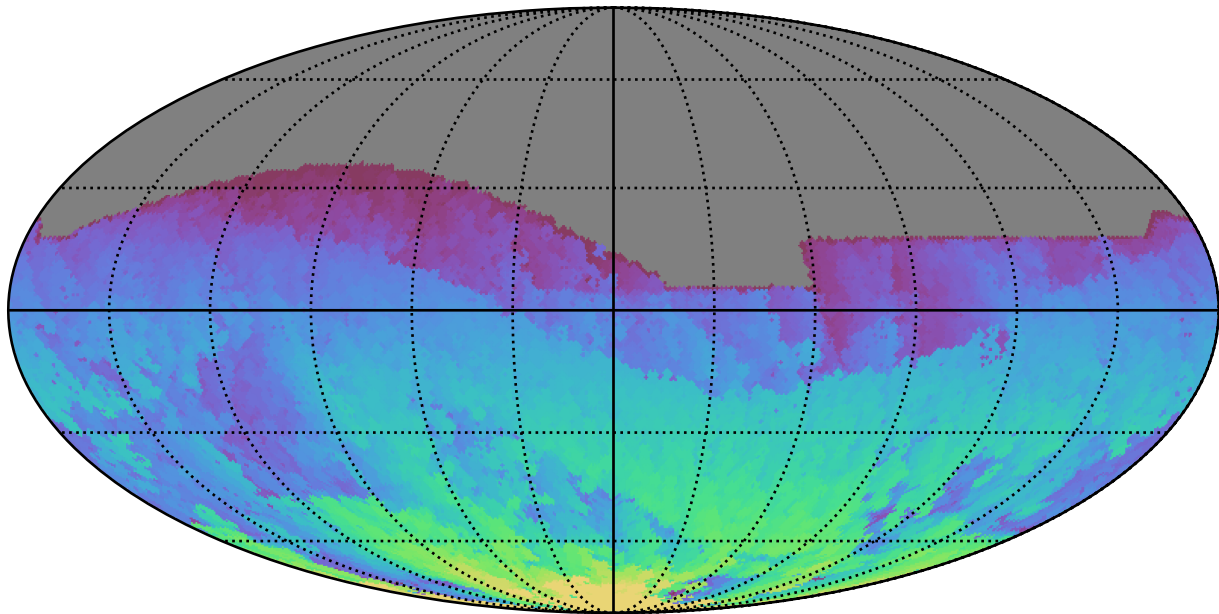
ddf_acor_sf10_lsf15_lsr10_v3.4_10yrs All sky i band: Max HA
