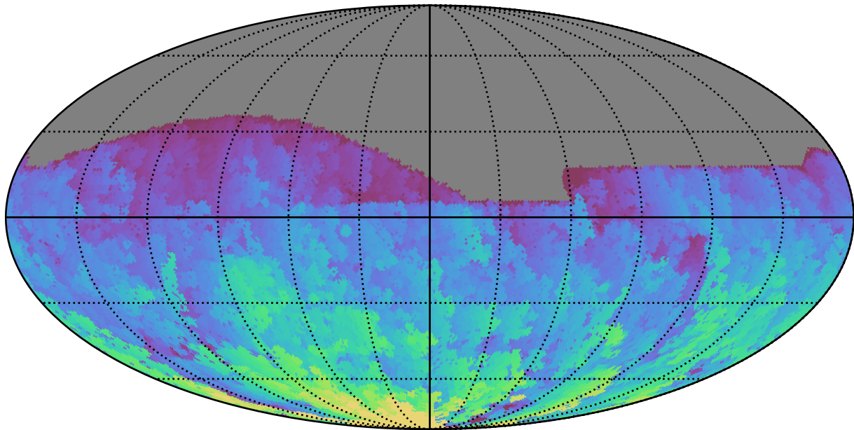
ddf_acor_sf10_lsf15_lsr10_v3.4_10yrs All sky g band: Max HA
