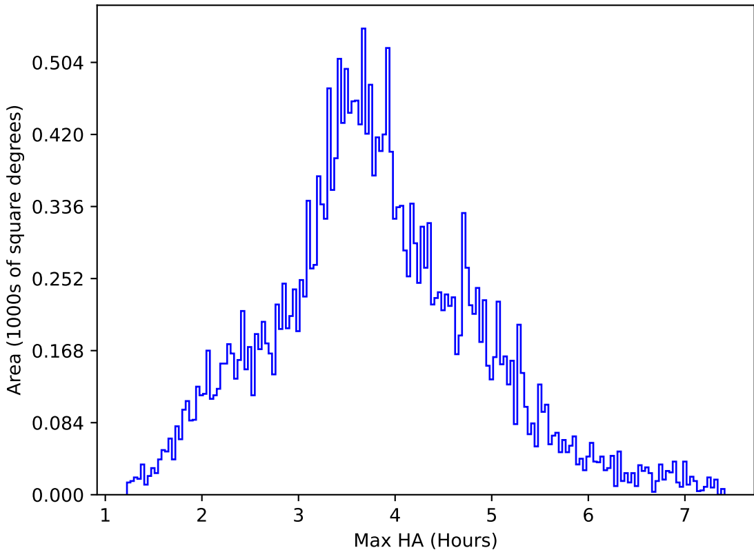
ddf_acor_sf10_lsf15_lsr10_v3.4_10yrs All sky g band: Max HA
