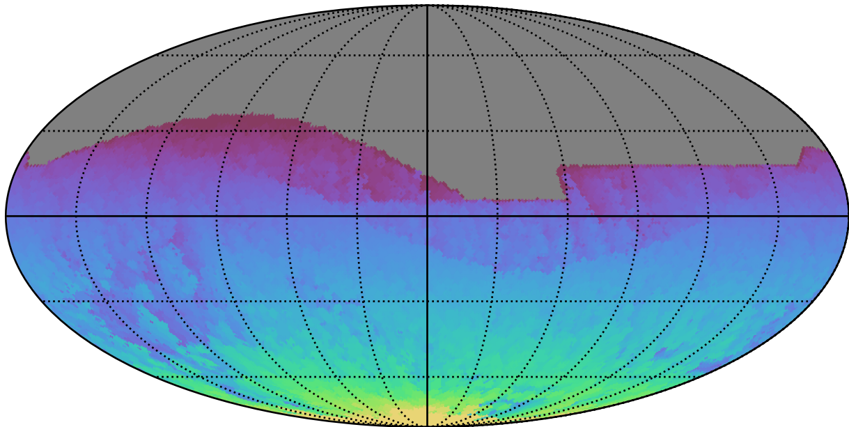
ddf_acor_sf10_lsf15_lsr10_v3.4_10yrs All sky all bands: Max HA
