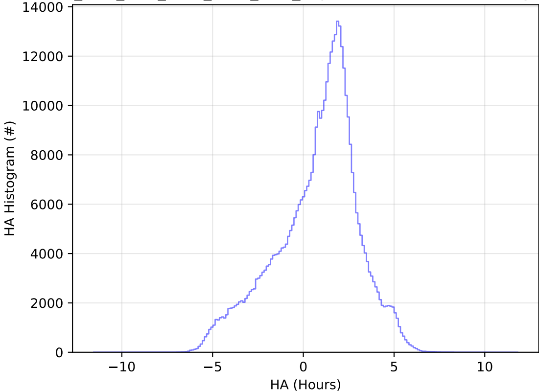
ddf_acor_sf10_ls15_lsr10_v3.4_10yrs WFD z band: HA Histogram
