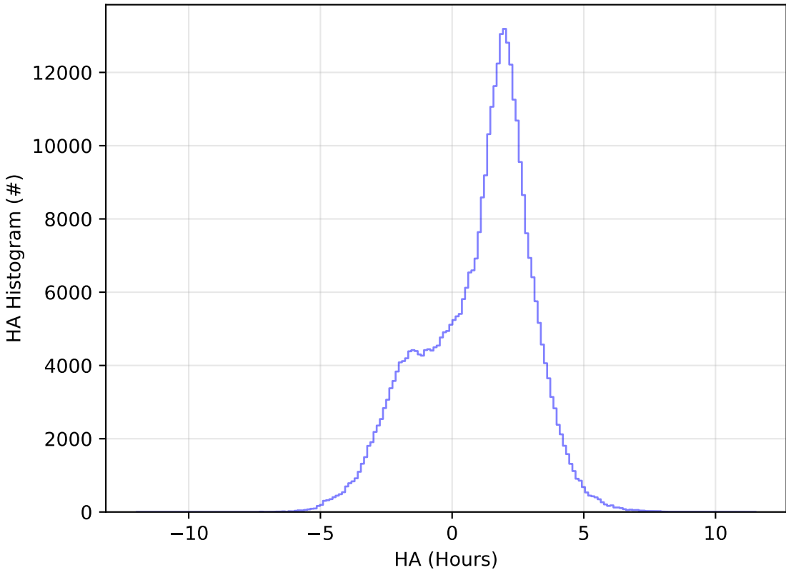
ddf_acor_sf10_lsf15_lsr10_v3.4_10yrs WFD y band: HA Histogram
