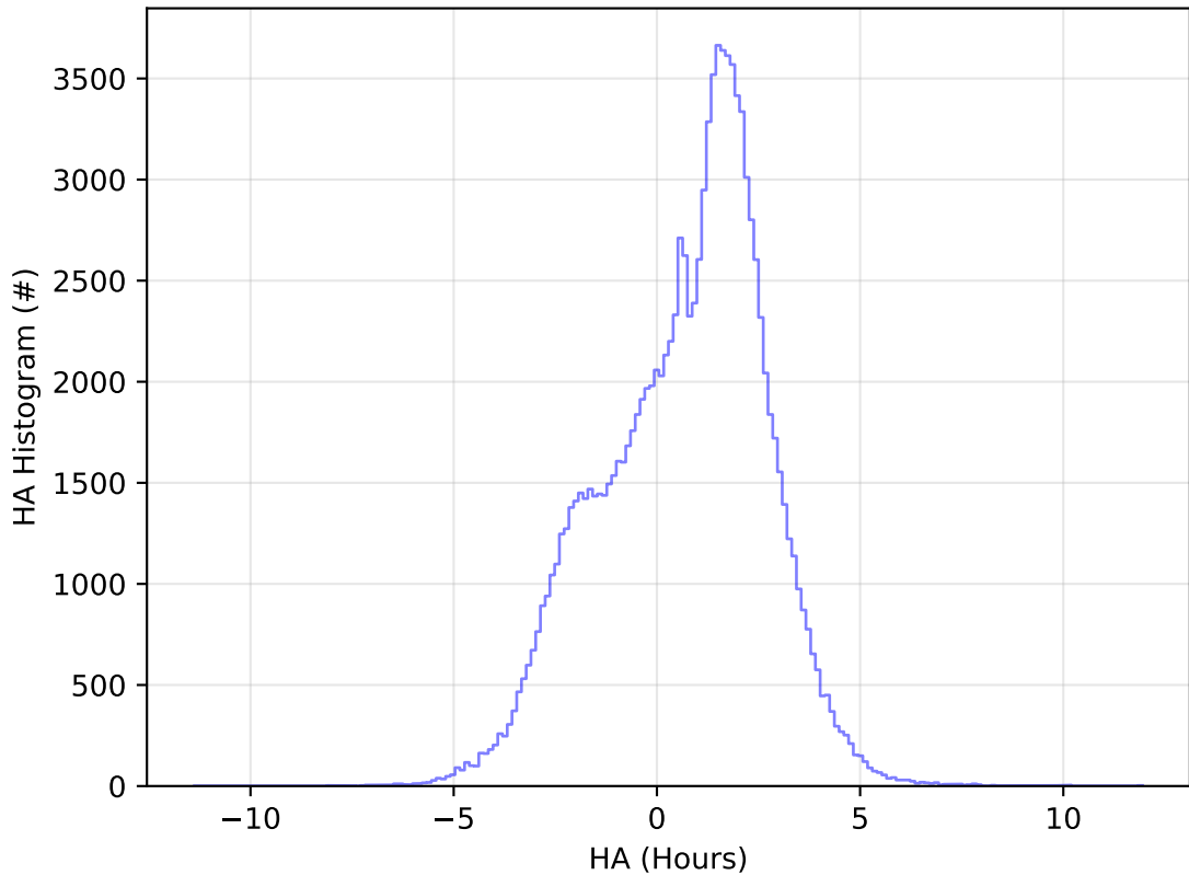
ddf_acor_sf10_lsf15_lsr10_v3.4_10yrs WFD u band: HA Histogram
