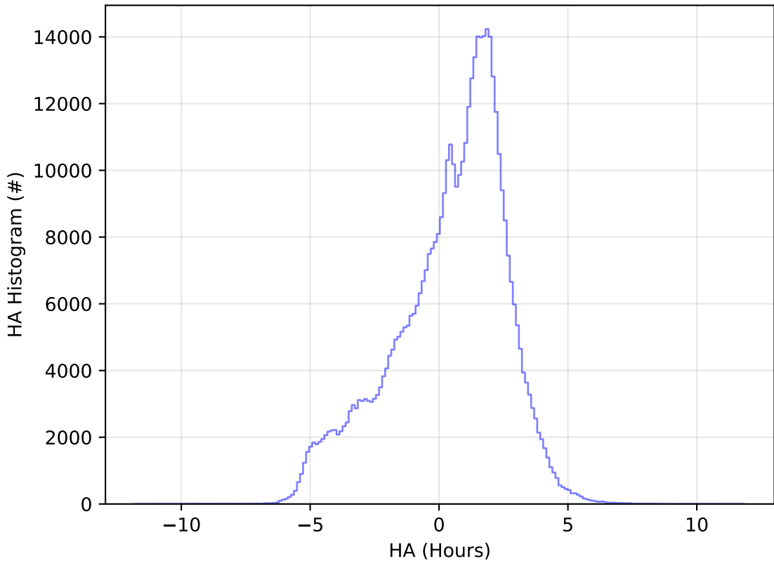
ddf_acor_sf10_lsf15_lsr10_v3.4_10yrs WFD r band: HA Histogram
