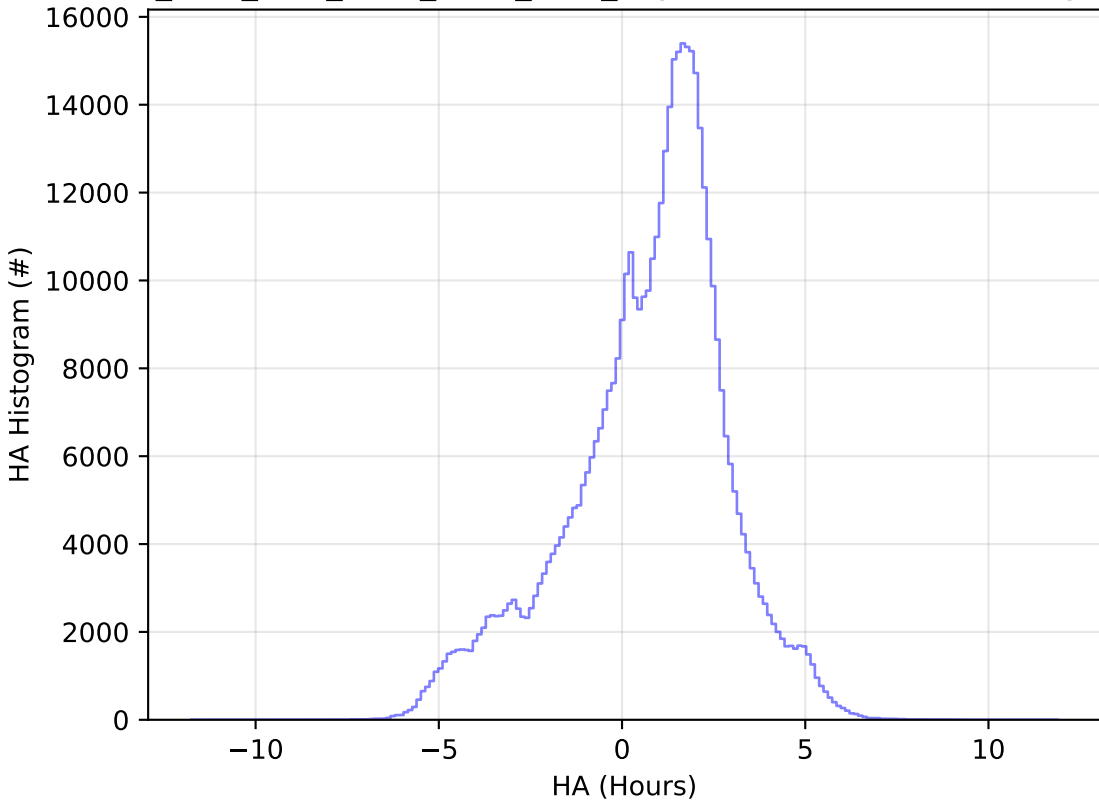
ddf_acor_sf10_lsf15_lsr10_v3.4_10yrs WFD i band: HA Histogram
