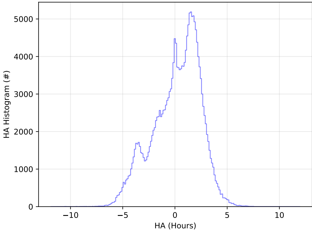
ddf_acor_sf10_lsf15_lsr10_v3.4_10yrs WFD g band: HA Histogram
