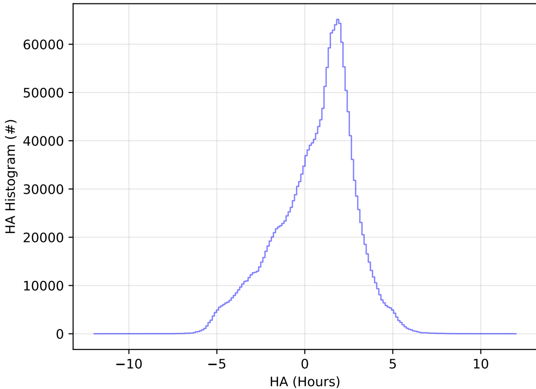
ddf_acor_sf10_ls15_lsr10_v3.4_10yrs WFD all bands: HA Histogram
