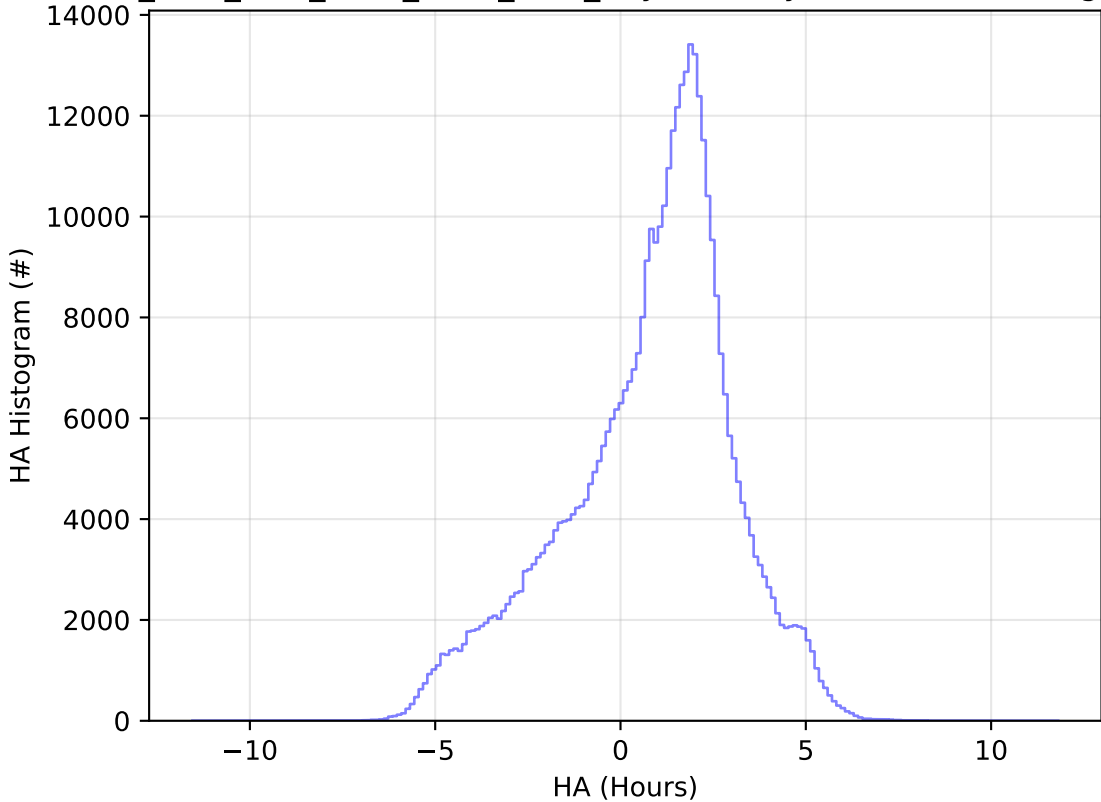
ddf_acor_sf10_lsf15_lsr10_v3.4_10yrs All sky z band: HA Histogram
