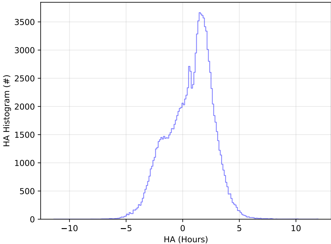
ddf_acor_sf10_lsf15_lsr10_v3.4_10yrs All sky u band: HA Histogram
