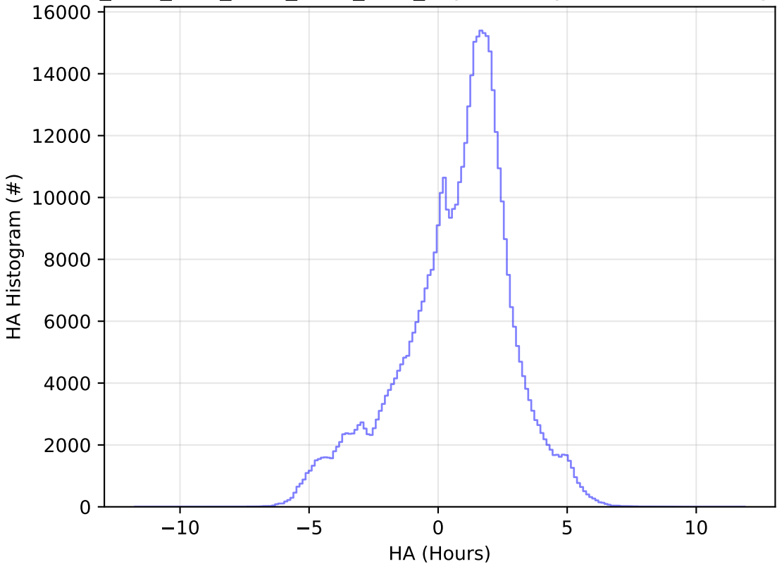
ddf_acor_sf10_lsf15_lsr10_v3.4_10yrs All sky i band: HA Histogram
