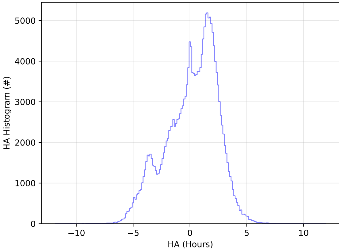
ddf_acor_sf10_lsf15_lsr10_v3.4_10yrs All sky g band: HA Histogram
