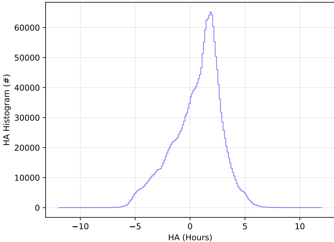
ddf_acor_sf10_lsf15_lsr10_v3.4_10yrs All sky all bands: HA Histogram
