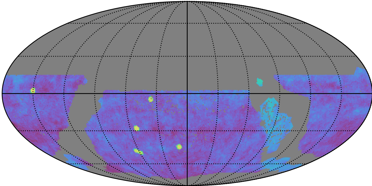
ddf_acor_sf10_ls15_lsr10_v3.4_10yrs gri WFD: Fraction of visits in pairs (10-60 min)
