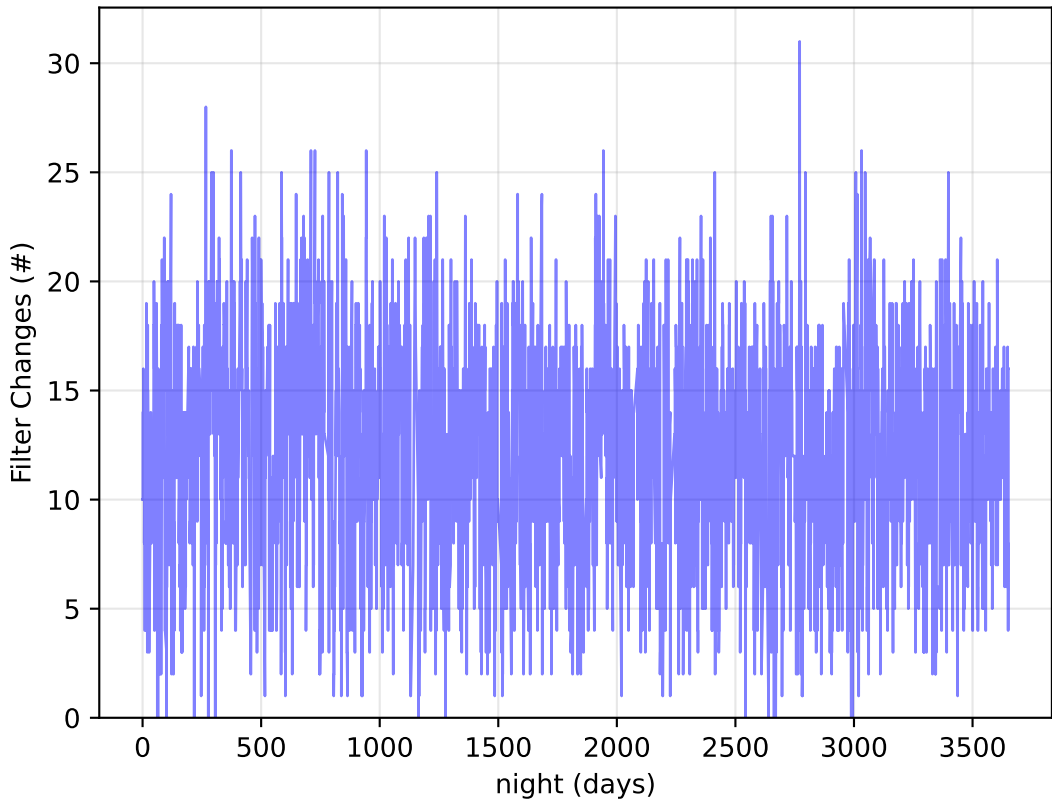
ddf_acor_sf10_lsf15_lsr10_v3.4_10yrs Per Night: Filter Changes
