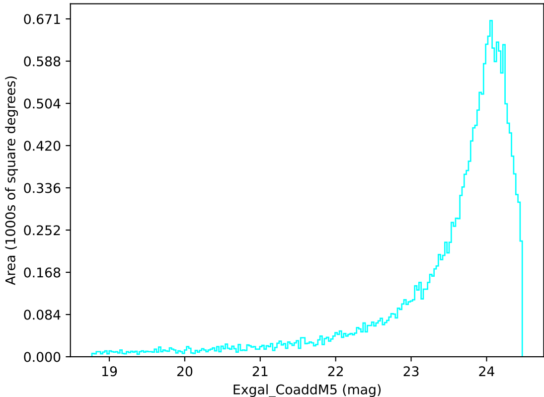
ddf_acor_sf10_lsf15_lsr10_v3.4_10yrs Yr 1 u band: Exgal_CoaddM5
