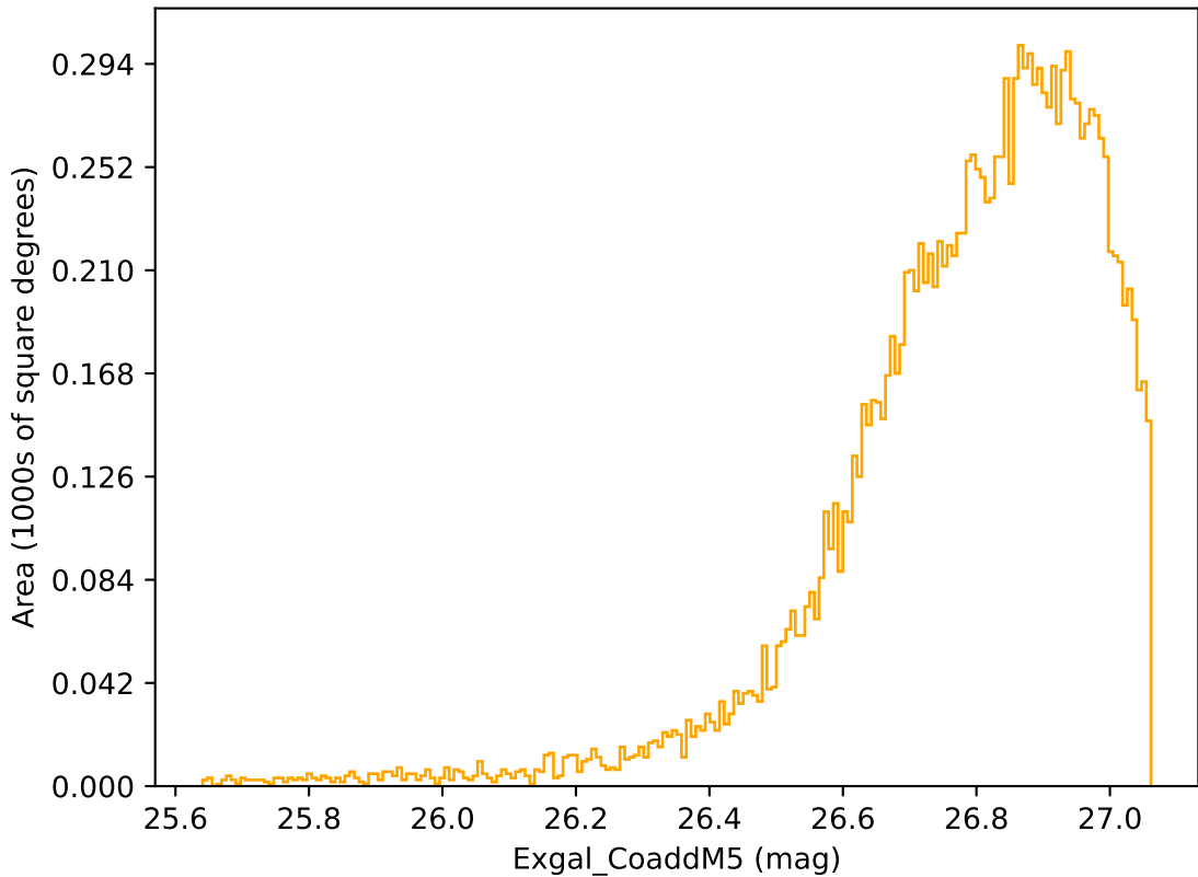
ddf_acor_sf10_lsf15_lsr10_v3.4_10yrs WFD r band: Exgal_CoaddM5
