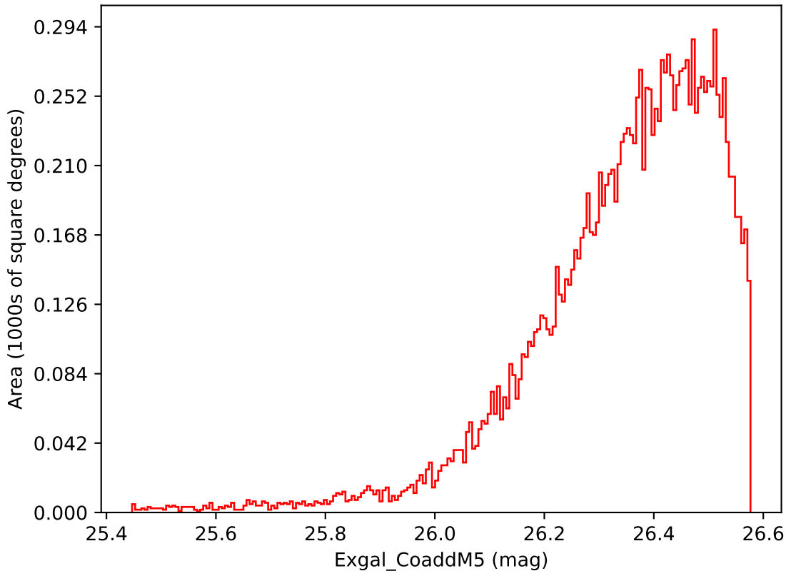
ddf_acor_sf10_lsf15_lsr10_v3.4_10yrs WFD i band: Exgal_CoaddM5
