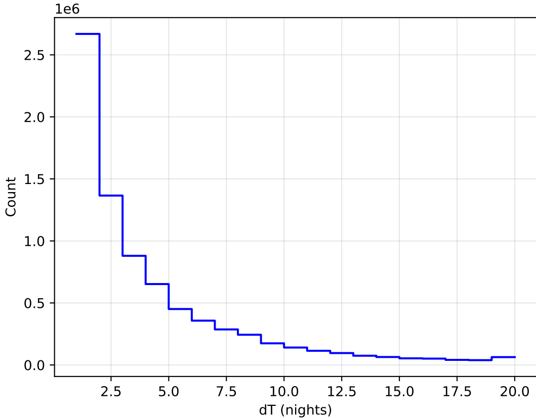
ddf_acor_sf10_lsf15_lsr10_v3.4_10yrs WFD all bands: DeltaNight Histogram
