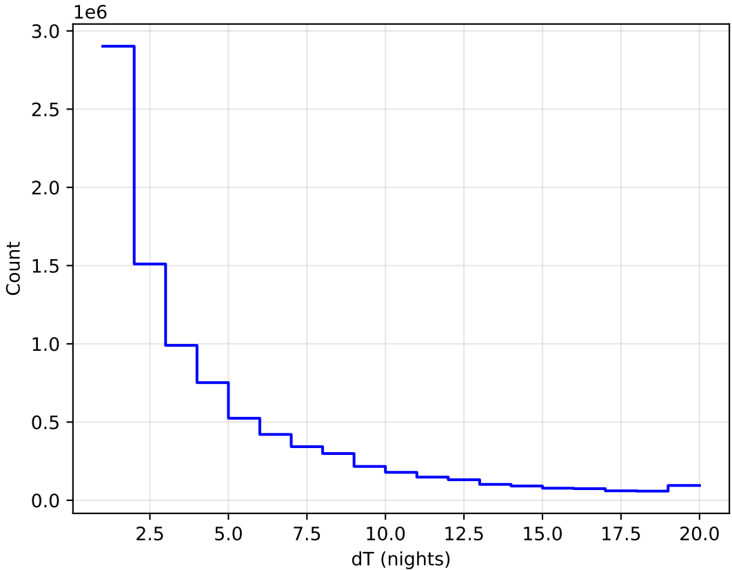
ddf_acor_sf10_lsf15_lsr10_v3.4_10yrs All sky all bands: DeltaNight Histogram
