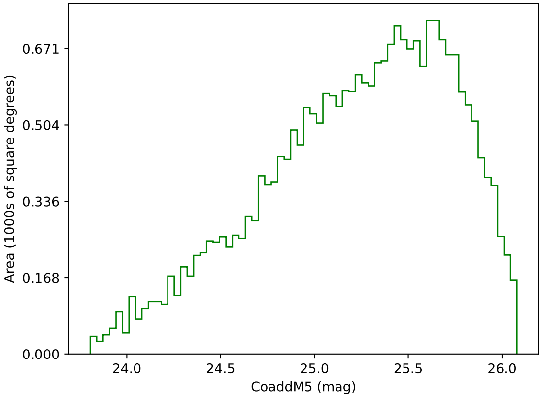
ddf_acor_sf10_lsf15_lsr10_v3.4_10yrs Yr 3-4 g band: CoaddM5
