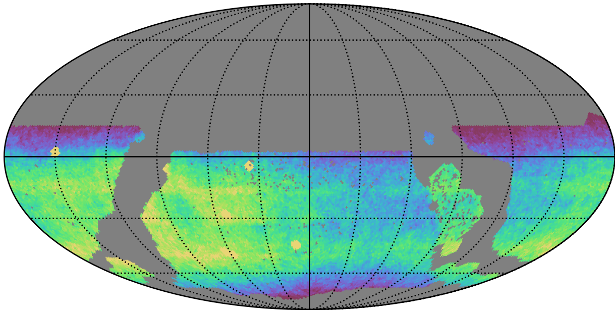
ddf_acor_sf10_lsf15_lsr10_v3.4_10yrs WFD r band: CoaddM5
