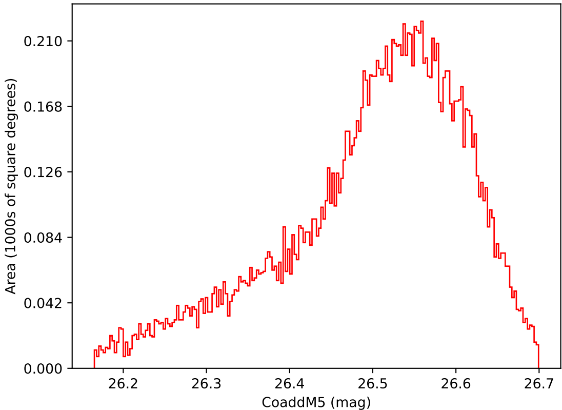
ddf_acor_sf10_lsf15_lsr10_v3.4_10yrs WFD i band: CoaddM5
