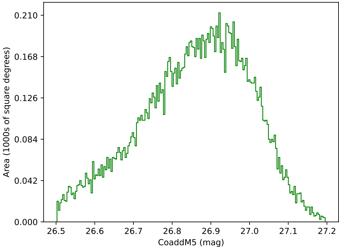
ddf_acor_sf10_lsf15_lsr10_v3.4_10yrs WFD g band: CoaddM5
