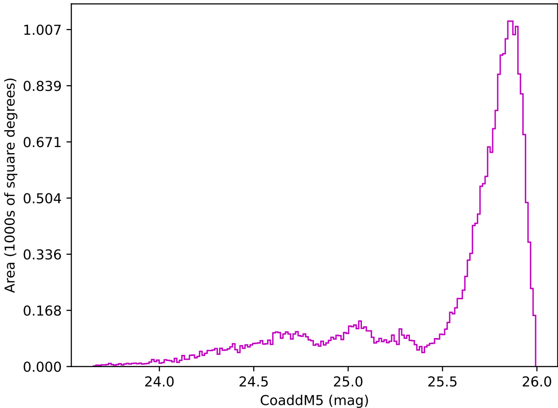
ddf_acor_sf10_lsf15_lsr10_v3.4_10yrs All sky z band: CoaddM5
