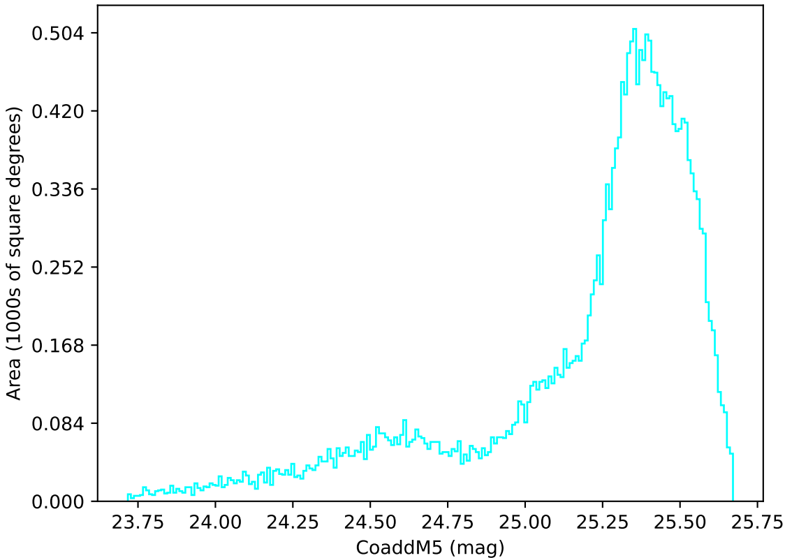
ddf_acor_sf10_lsf15_lsr10_v3.4_10yrs All sky u band: CoaddM5
