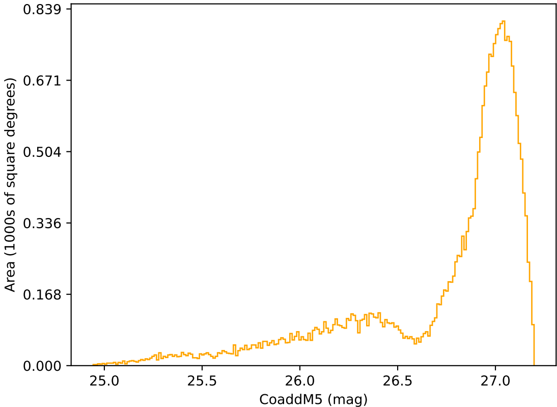
ddf_acor_sf10_lsf15_lsr10_v3.4_10yrs All sky r band: CoaddM5
