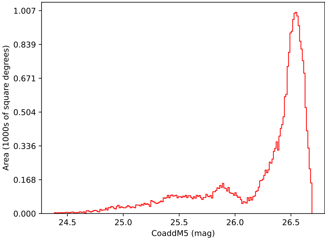
ddf_acor_sf10_lsf15_lsr10_v3.4_10yrs All sky i band: CoaddM5
