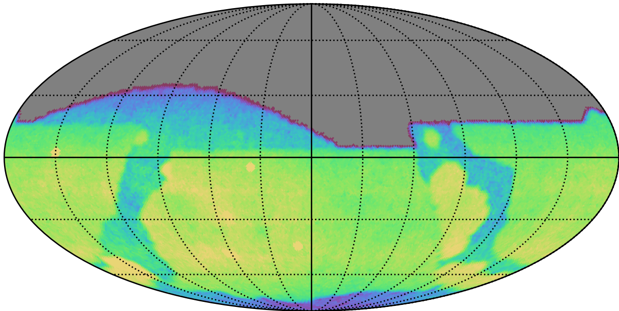
ddf_acor_sf10_lsf15_lsr10_v3.4_10yrs All sky g band: CoaddM5
