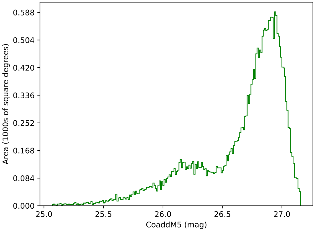
ddf_acor_sf10_lsf15_lsr10_v3.4_10yrs All sky g band: CoaddM5
